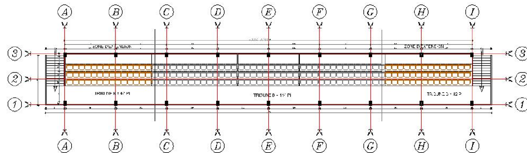
Plan ETAGE Existant 114 PLACES Extension 84 Places
