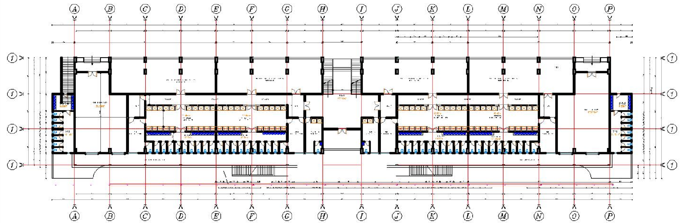
Plan R D C Ech:1/100
